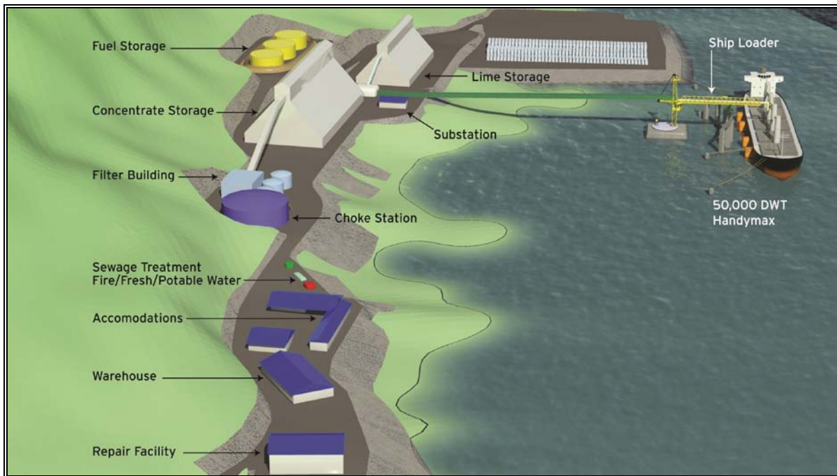
Figure 1.9.1 Port Site 1 Layout
