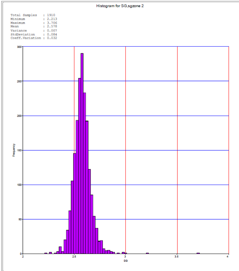
Figure 17.4.2 Representative Histograms of Density Data for SGZONE 2 and SGZONE 3
