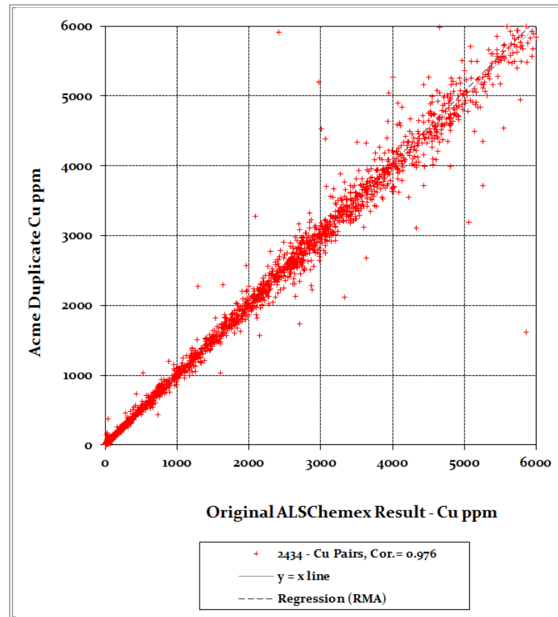
Figure 14.1.4 Comparison of Copper Duplicate Assay Results for 2005-2010
