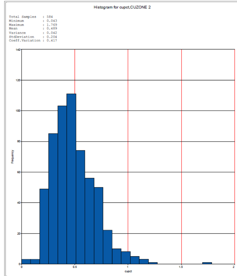
Figure 17.3.1 Histograms for Copper (CUZONE 2) – Raw Data and Compositied Data
