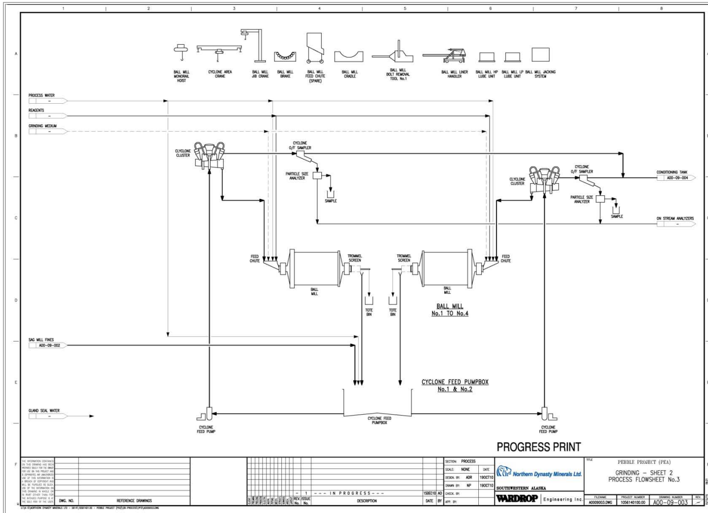
Figure 16.13.3 Grinding Process Flowsheet – Sheet 2
