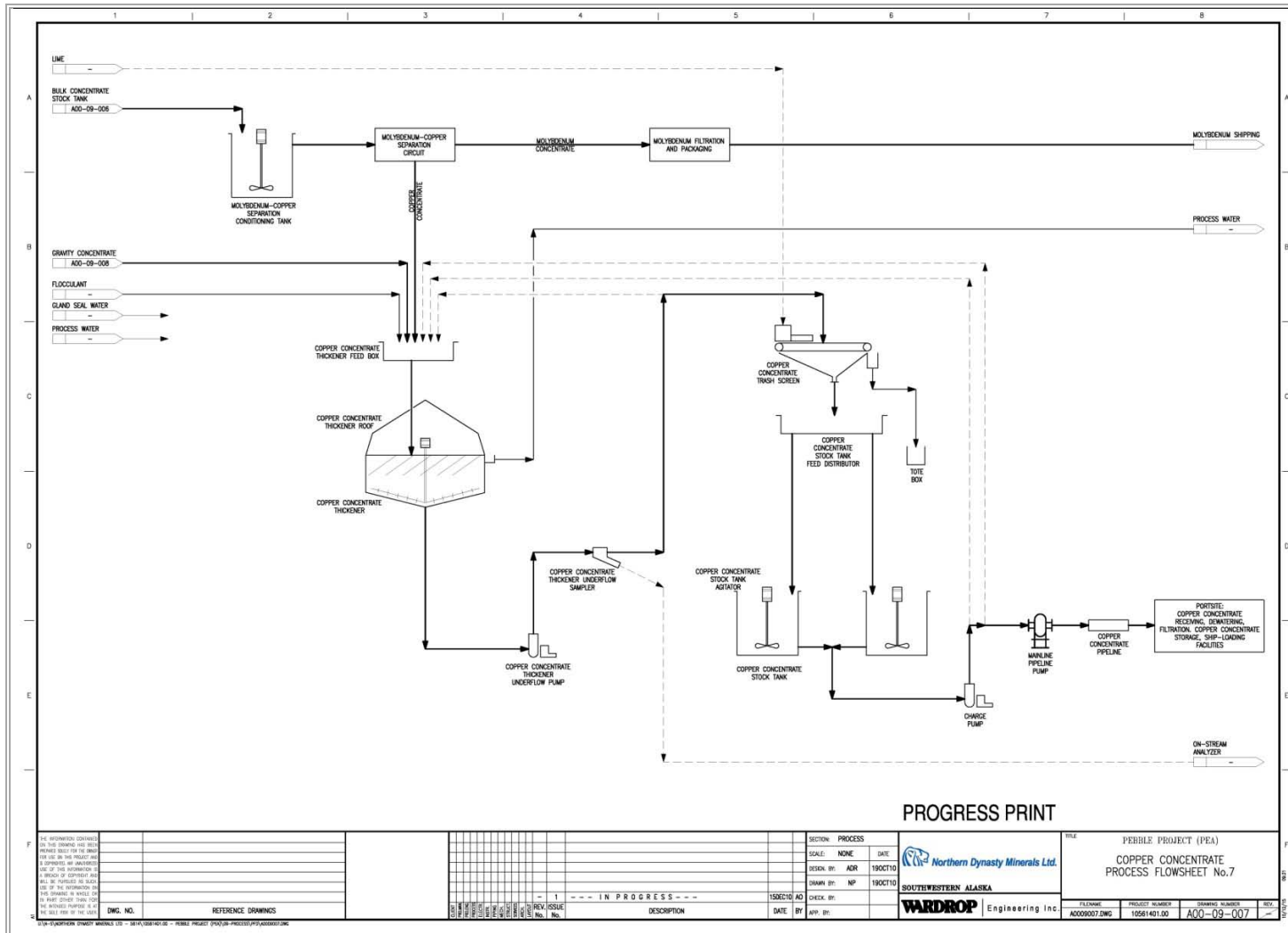
Figure 16.13.7 Copper Concentrate Process Flowsheet
